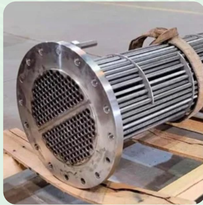
Extractor Condenser & Heater Tube
